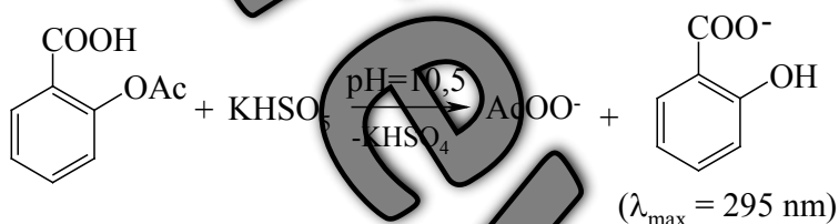
Scheme 10. Perhydrolysis reaction of aspirin by means of potassium peroxymonosulfate.
