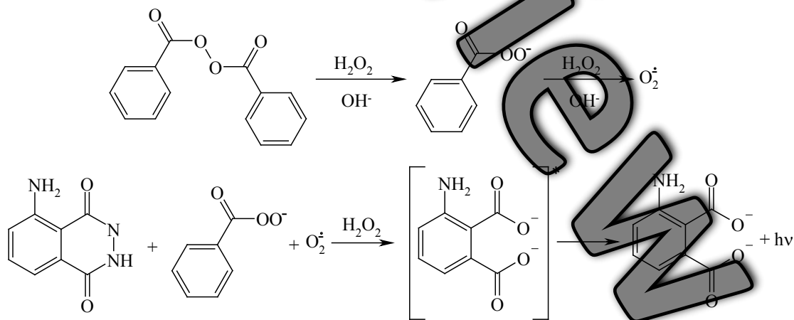
Scheme 14. Perhydrolysis of benzoyl peroxide and coupled Luminol peroxyacid oxidation reaction.
