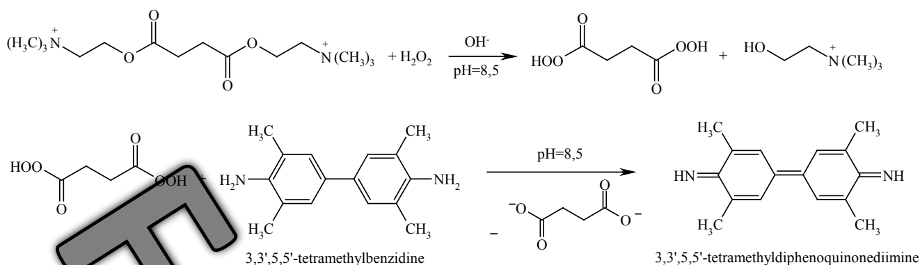
Scheme 12. Chemistry of SUX perhydrolysis and coupled TMB peroxyacid oxidation.
