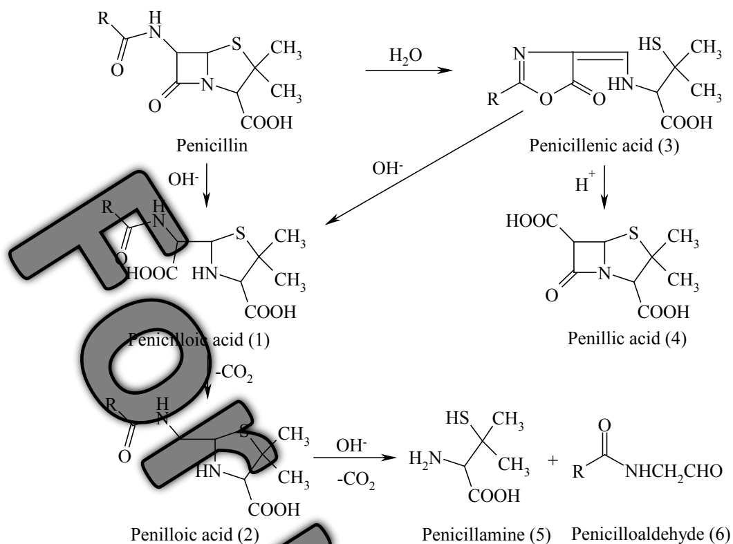
Scheme 1. Known degradation behavior of penicillins under different hydrolytic conditions.
