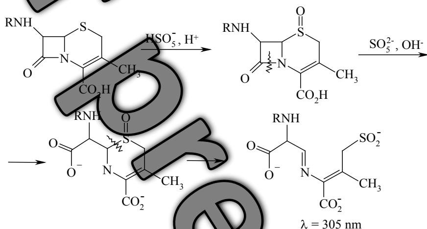
Scheme 4. Mechanism of Cephalexin chemical transformations by means of potassium peroxomonosulfate and alkali.
