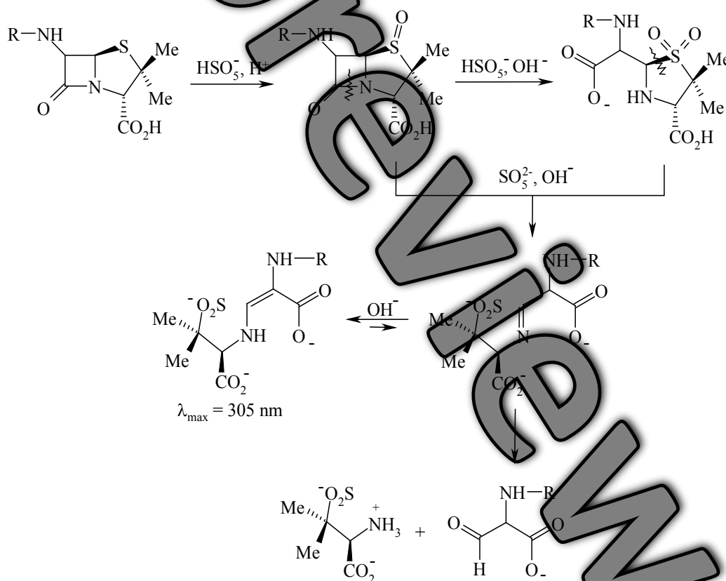
Scheme 3. Mechanism of Ampicillin chemical transformations by means of potassium peroxomonosulfate in alkali medium.
