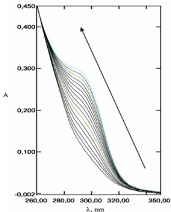
Fig.3. Electronic spectra of product perhydrolysis of DL -lysine acetylsalicylate, obtained by means of potassium peroxomonosulfate (for 30 minutes, every 2 minutes, starting at 30 seconds): c(\text{DL-lysine acetylsalicylate}) = 28.8 \mu\text{g mL}^{-1} ; c(\text{KHSO}_5) = 3.6 \cdot 10^{-3} \text{ mol L}^{-1} ; \text{pH} = 10.5 .
