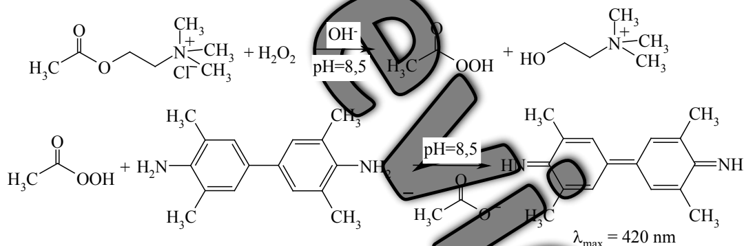
Scheme 6. Chemistry of Acetylcholine perhydrolysis and coupled TMB peroxoacid oxidation.
