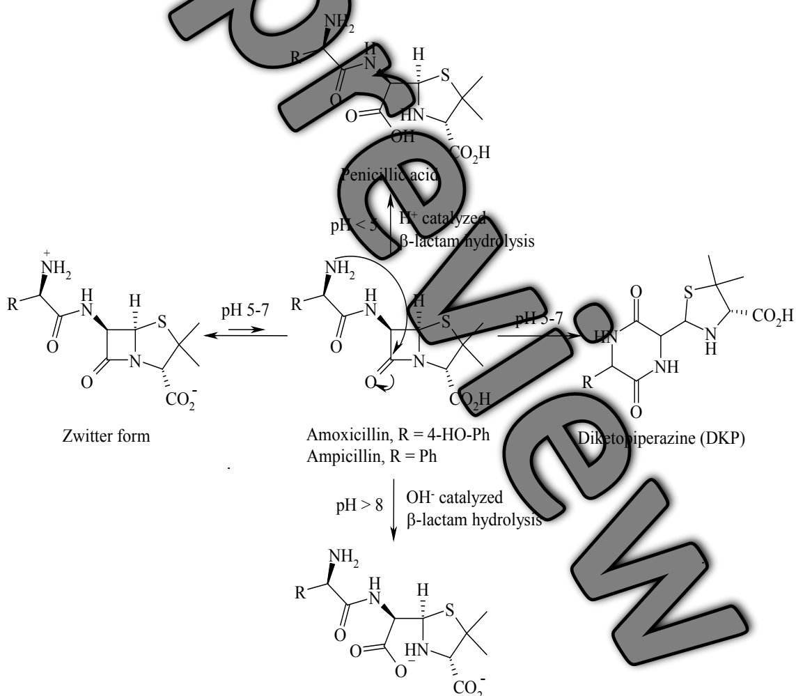
Scheme 2. Major degradation pathways of aminopenicillins under of different pH ranges.
