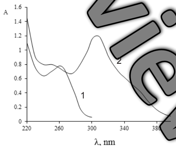
Fig. 2. Electronic spectra of Cephalexin absorption (1) and product of conjugated reactions of S-oxidation and perhydrolysis with potassium peroxomonosulfate (2). c(\text{Cph}) = 1 \cdot 10^{-4} \text{ mol L}^{-1} ; c(\text{KHSO}_5) = 2 \cdot 10^{-4} \text{ mol L}^{-1} ; c(\text{NaOH}) = 0.01 \text{ mol L}^{-1} .
