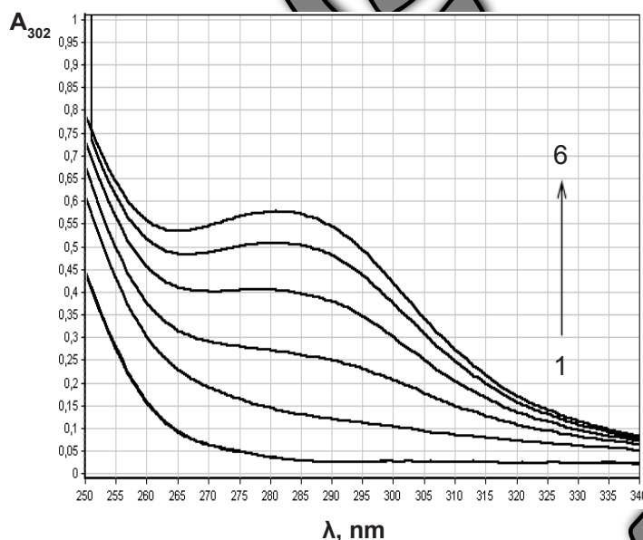
Fig. 1. Electronic spectra of light absorbance of the products of alkaline hydrolysis (1) and perhydrolysis of sodium oxacillin (2-6) in the time, min: 1) 0-20, 2) 5, 3) 10, 4) 15, 5) 20, 6) 25; c(\text{NaOH}) = 6.1 \cdot 10^{-3}\text{ mol L}^{-1} ; c(\text{KHSO}_5) = 1.2 \cdot 10^{-3}\text{ mol L}^{-1} ; c(\text{Na-oxac.}) = 30\text{ }\mu\text{mol mL}^{-1} .
