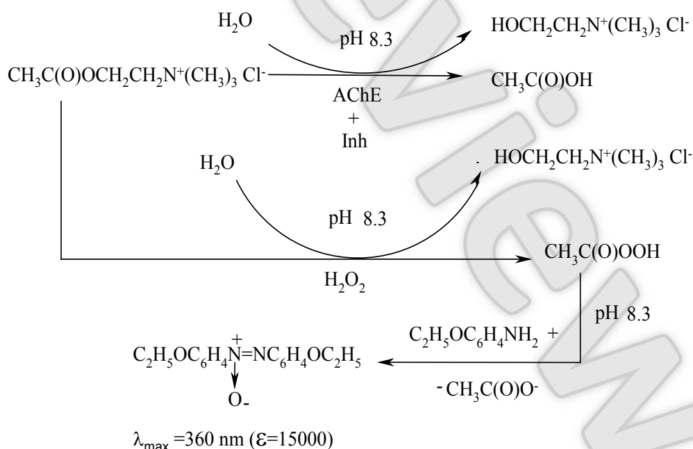
Fig. 1. The scheme of processes of the analytical determination.
