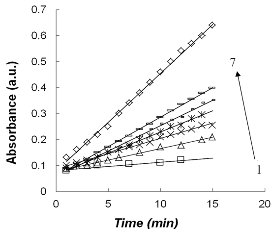
Fig.2. Kinetic curves of couple oxidation of p -phenetidine by hydrogen peroxide in the system: 1 – \text{ACh} + \text{ChE} , 2– 6 – \text{ACh} + (\text{ChE} + \text{BAC}) , 7 – \text{ACh} . w(\text{ACh}) = 0.1\% ; [\text{ChE}] = 0.25 \text{ U} ; c(\text{BAC}), 10^{-6} \text{ M} : 2–1.4, 3–2.8, 4–3.4, 5–5.6, 6–7.0.
