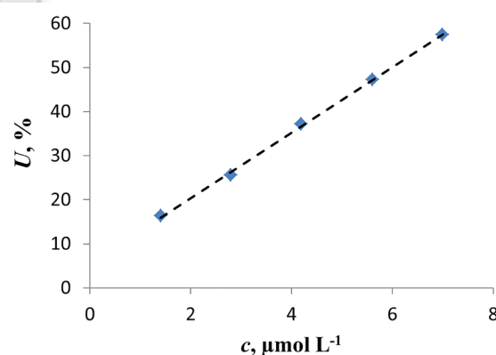
Fig.3. Curve of the graduated dependence of inhibition degree vs BAC concentrations.
