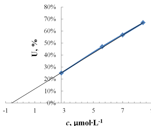
Fig. 4. Results of Recovery Study Using Standard-Addition method.
